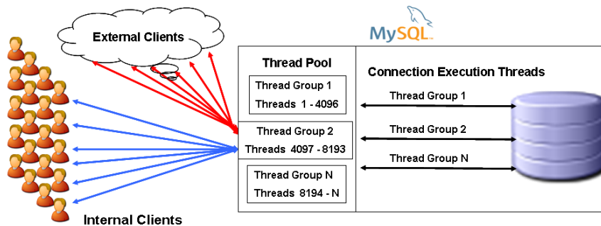
Figure 5: MySQL Thread Pool
