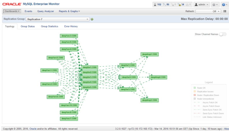
Figure 12: Multi-source Replication topology view
