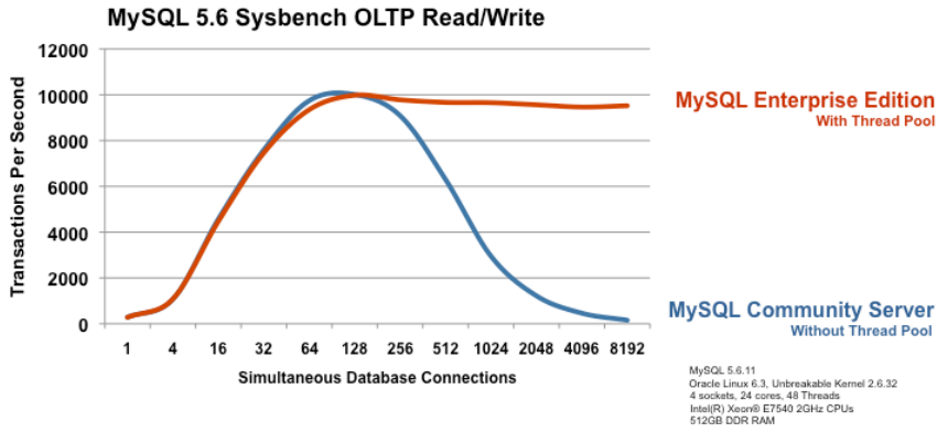
Figure 6: MySQL Enterprise Edition provides 60x better scalability for OLTP Read/Write activity with Thread Pool
