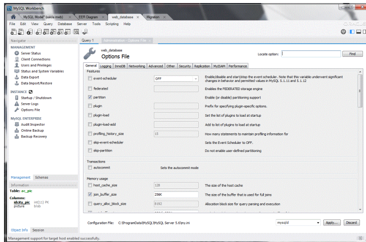
Figure 21: MySQL Workbench – Server Administration, Monitoring
