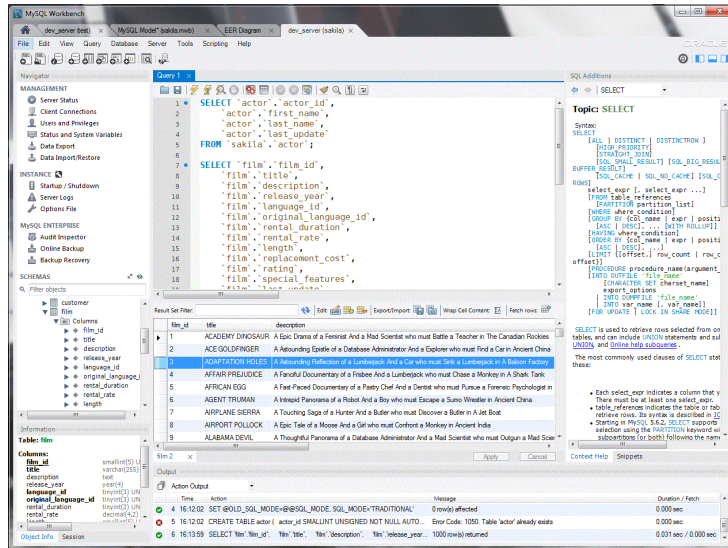
Figure 20: MySQL Workbench – SQL Development, Execution, Tuning
