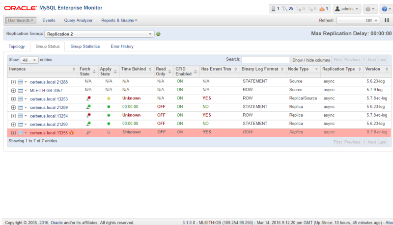
Figure 13: MySQL Replication Group Status View
