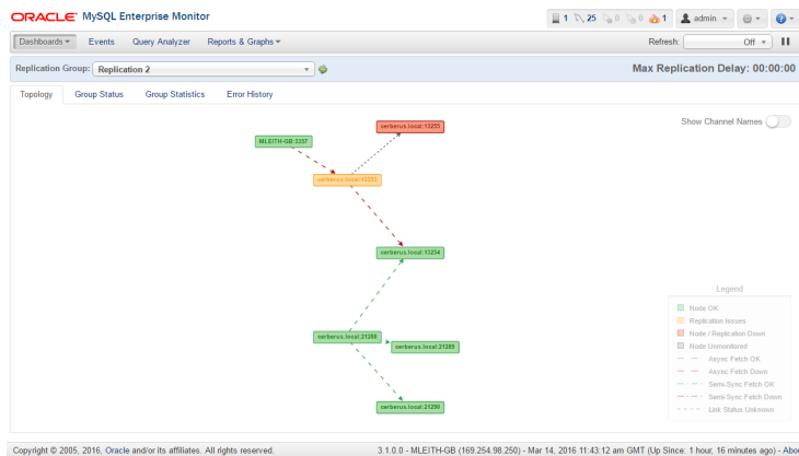
Figure 11: MySQL Enterprise Replication Dashboard topology view
