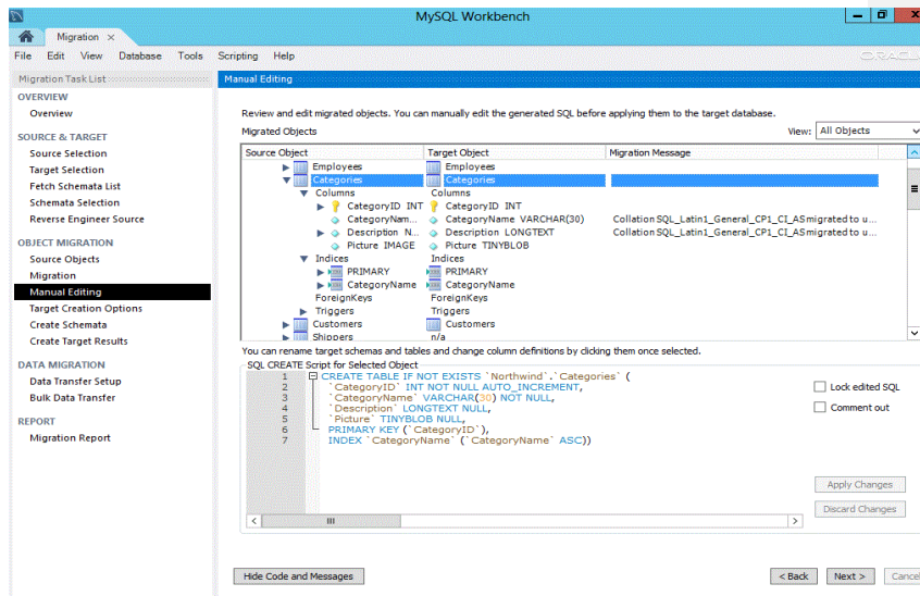
Figure 22: MySQL Workbench – Database Migration Wizard
