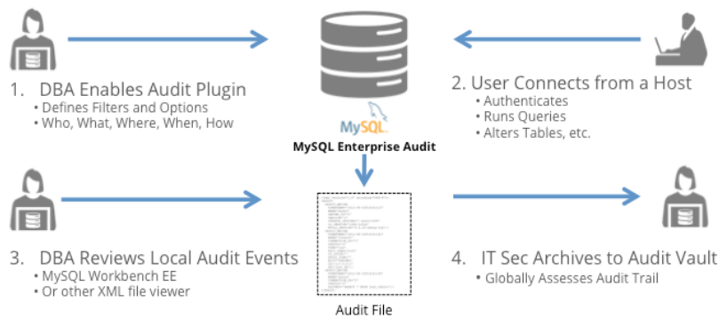
Figure 1: MySQL Enterprise Audit Set Up and Use Case
