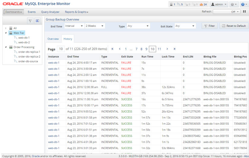
Figure 15: MySQL Enterprise Backup Dashboard History View
