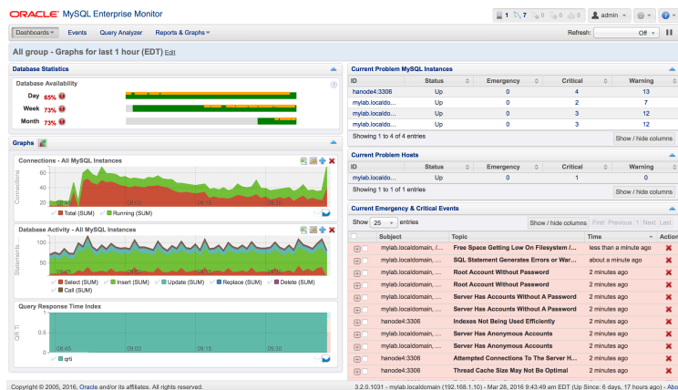
Figure 10: MySQL Enterprise Dashboard
