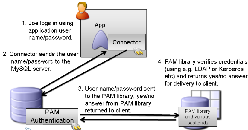
Figure 2: MySQL External Authentication for PAM
