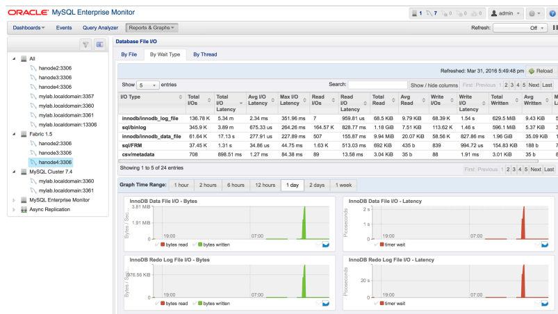
Figure 17: MySQL Database File I/O – By Wait Type
