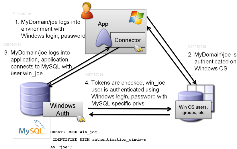
Figure 3: MySQL External Authentication for Windows
