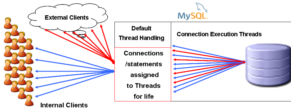
Figure 4: Default Thread Handling Model
