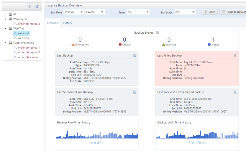
Figure 14: MySQL Enterprise Backup Dashboard Instance View
