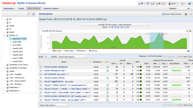
Figure 16: MySQL Query Analyzer
