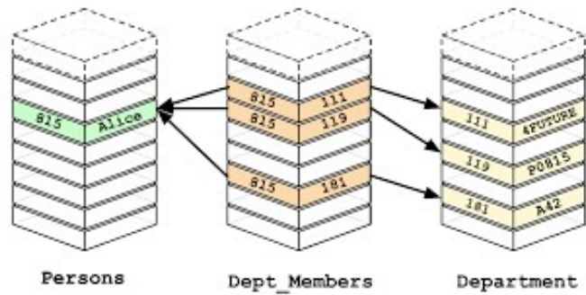
Relational Database
