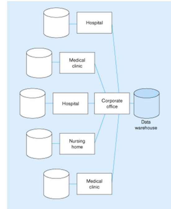
Enterprise Database
