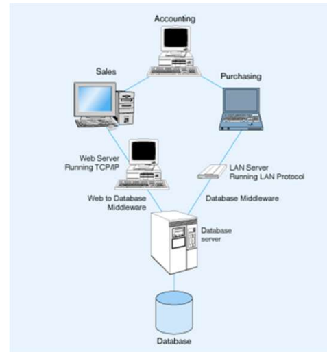
Department Database
