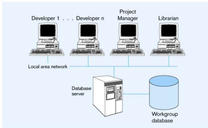
Workgroup Database
