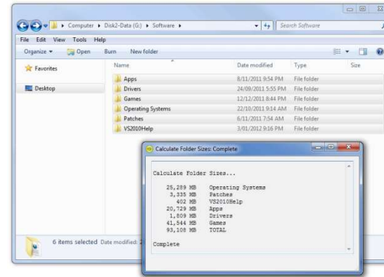
Hierarchical Database
